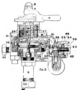
Fig. 2472. Section.
